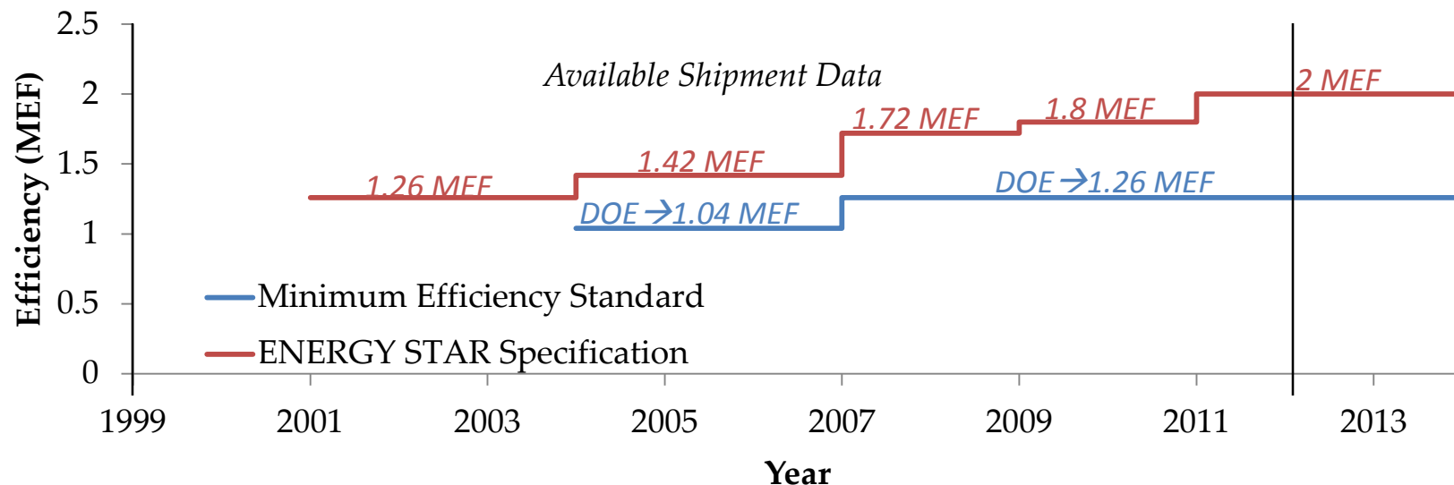
Figure 17—Historical Efficiency Standards
