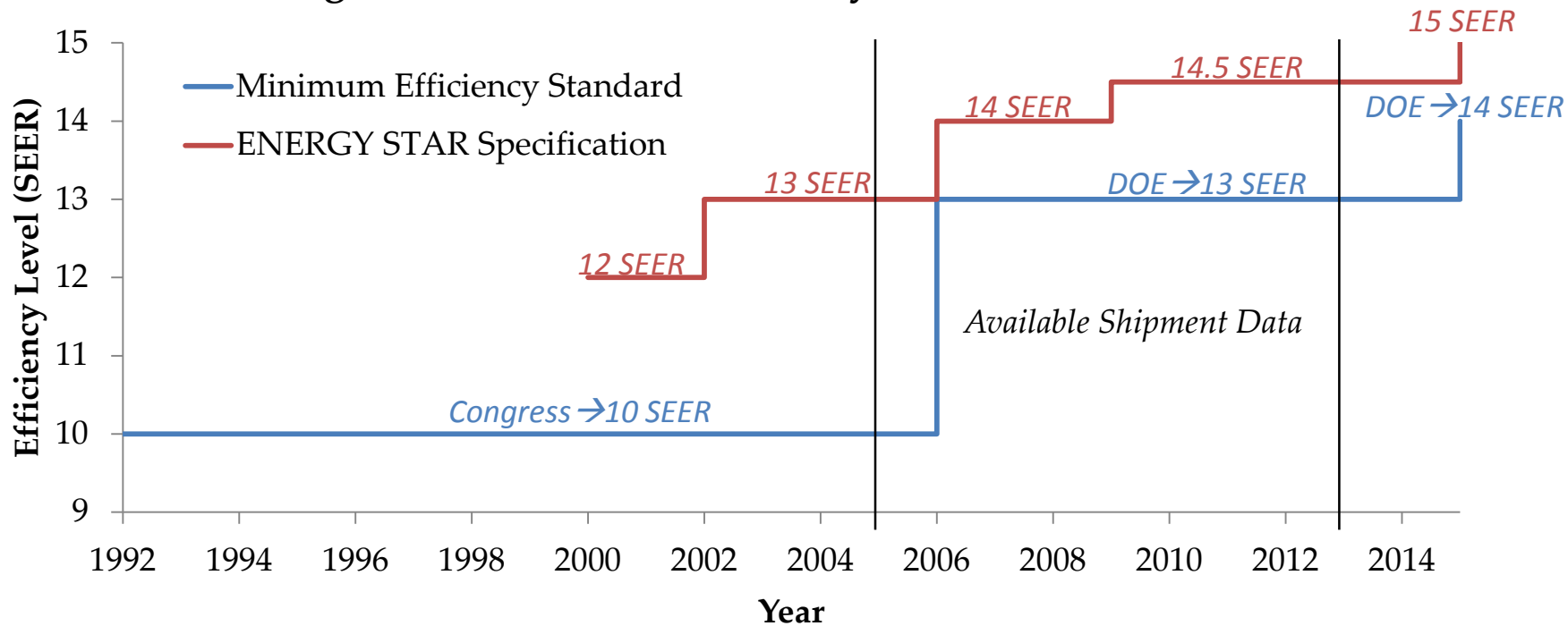
Figure 10—Historical Efficiency Standards (SEER)
