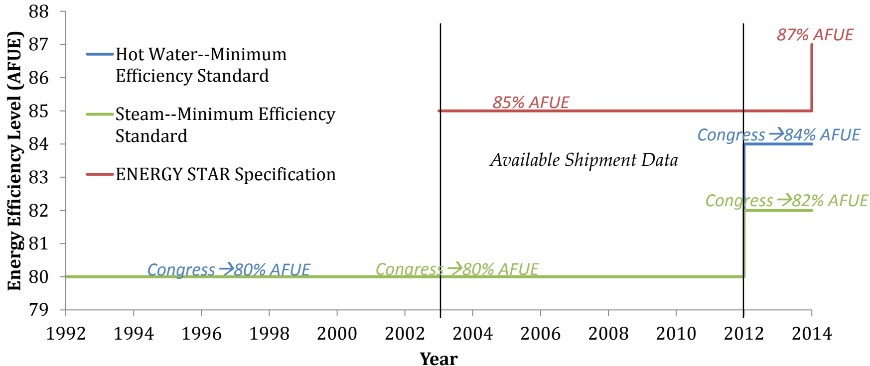
Figure 35—Historical Efficiency Standards
