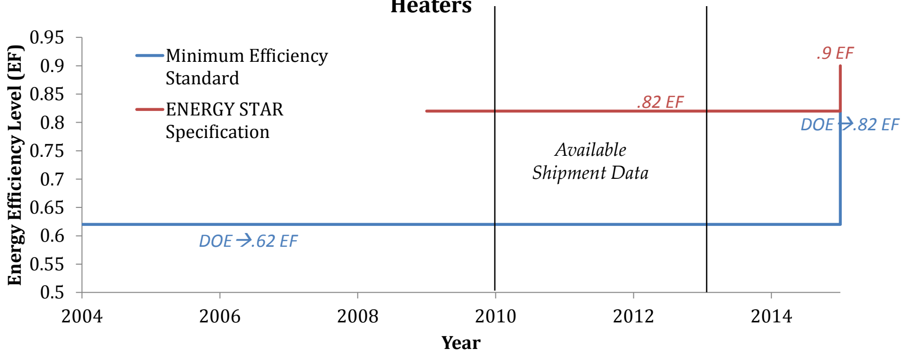
Figure 7—Historical Efficiency Standards for Instantaneous Water Heaters
