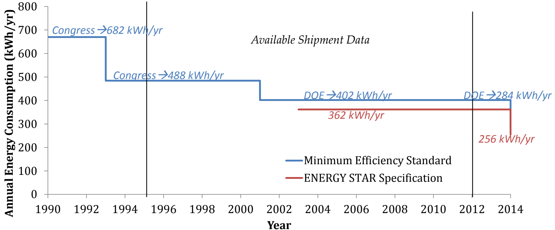
Figure 24—Historical Efficiency Standards
