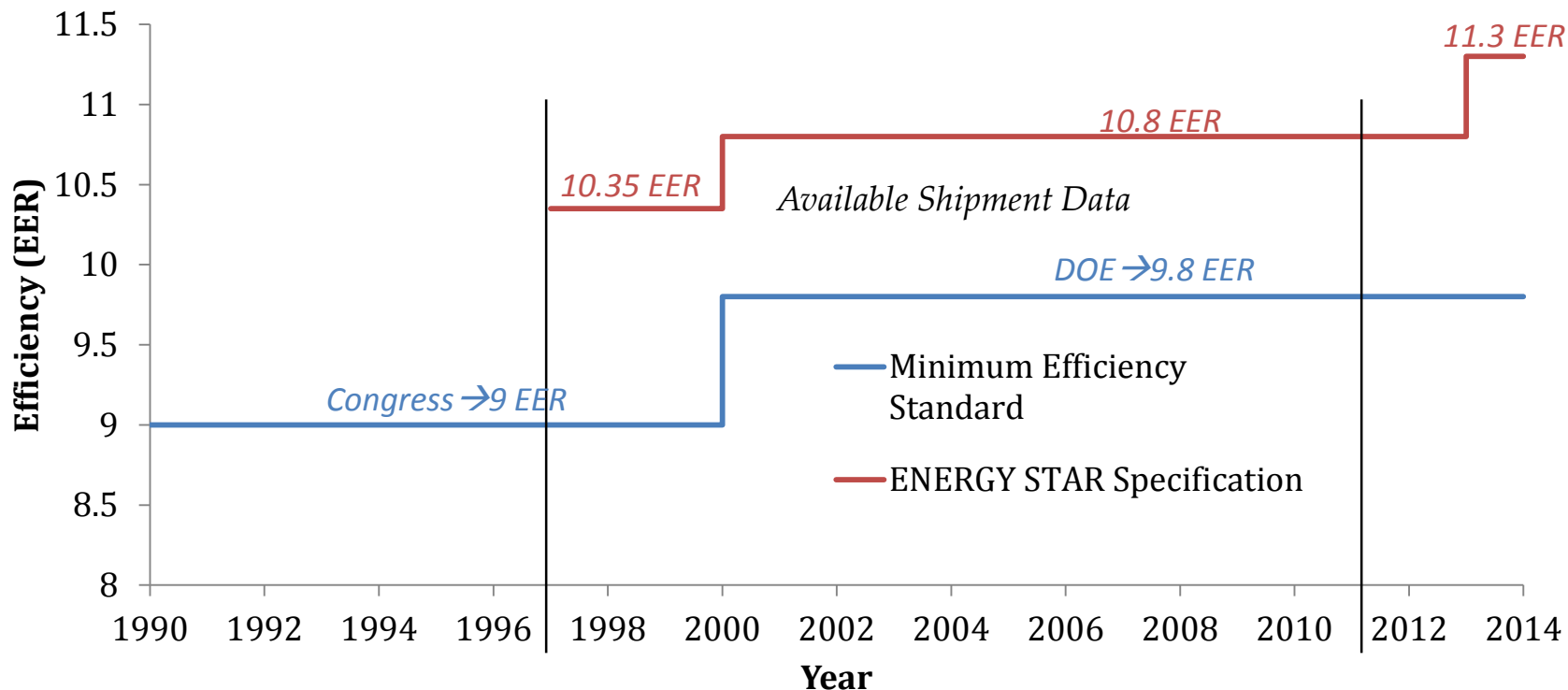
Figure 15—Historical Efficiency Standards
