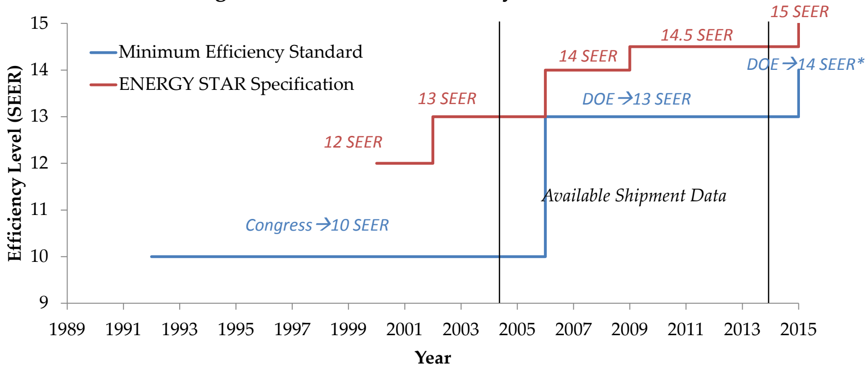
Figure 13—Historical Efficiency Standards
