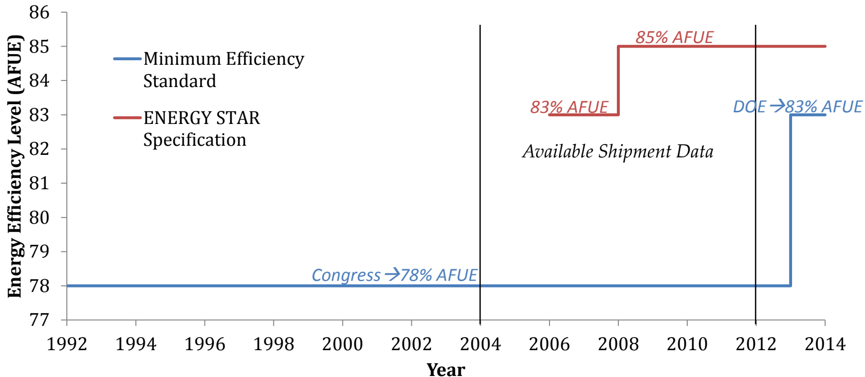
Figure 33—Historical Efficiency Standards
