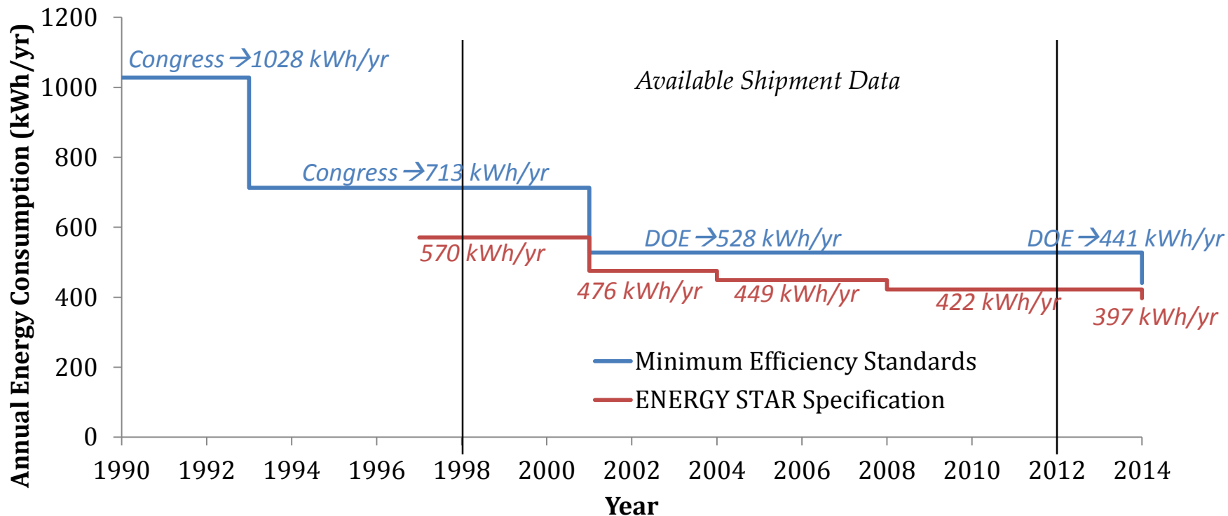
Figure 22—Historical Efficiency Standards
