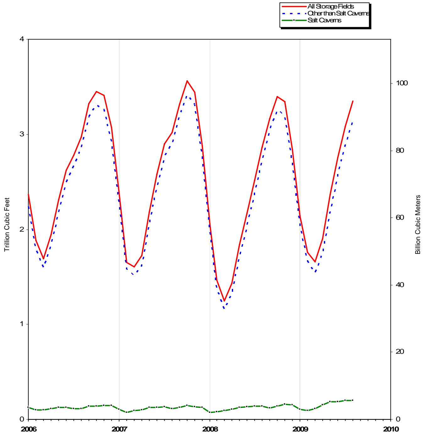
Figure 5. Working Gas in Underground Natural Gas Storage in the United States, 2006-2009
