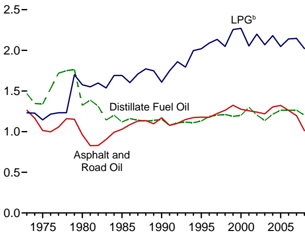
Transportation Sector, 1973-2008
