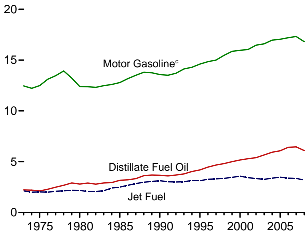
Transportation Sector, 1973-2008
