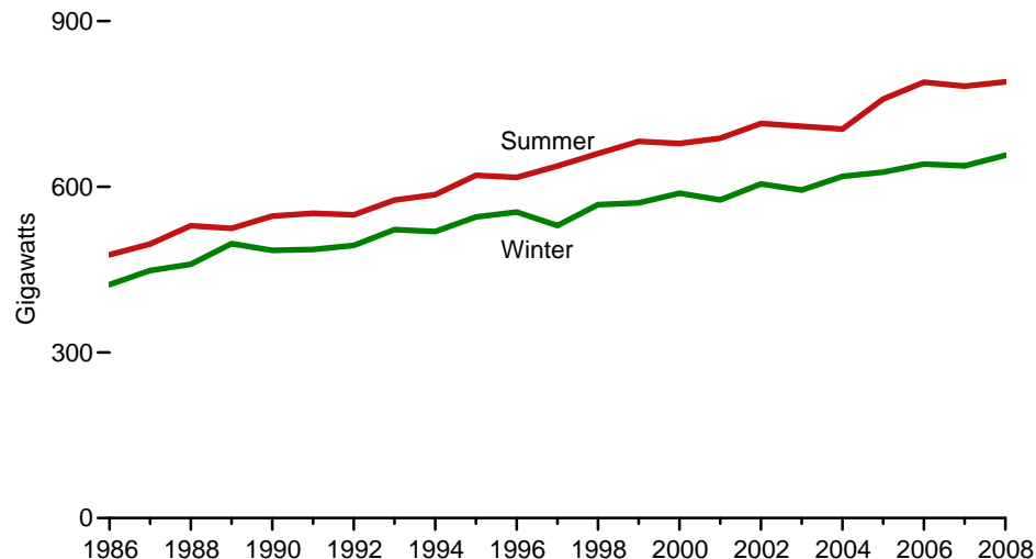
U.S. Peak Load, 1986-2008
