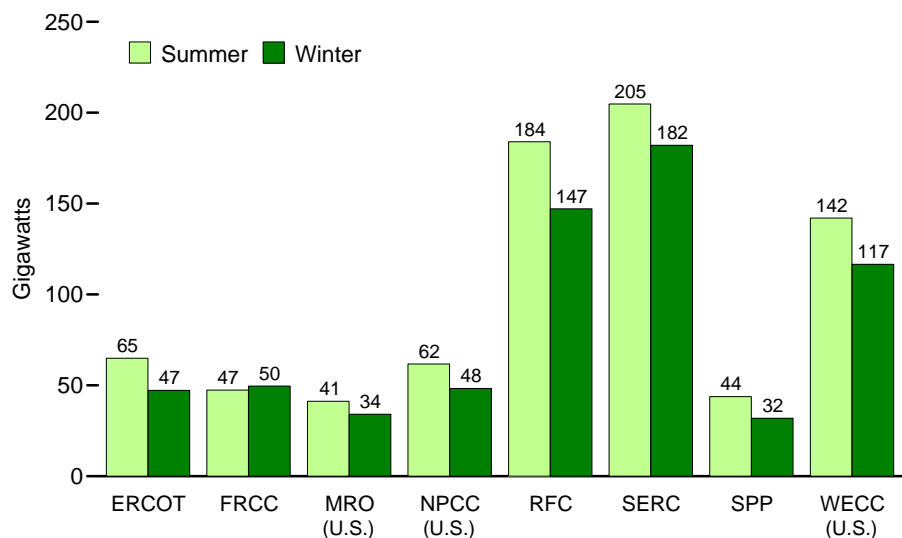
U.S. Peak Load by NERC Region, 2008
