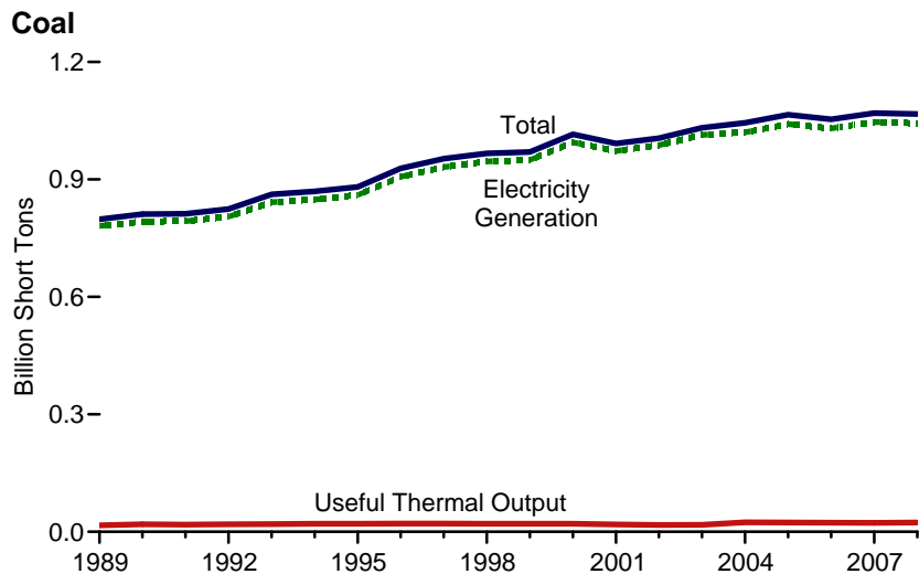
Figure 8.7 Consumption of Combustible Fuels for Electricity Generation and Useful Thermal Output, 1989-2008
