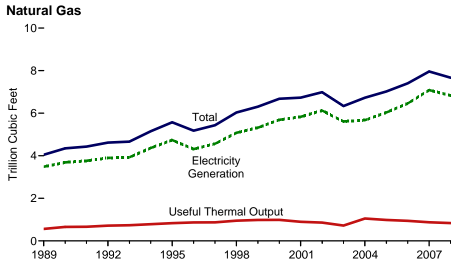
Figure 8.7 Consumption of Combustible Fuels for Electricity Generation and Useful Thermal Output, 1989-2008
