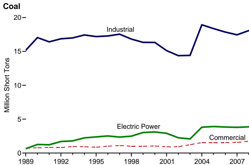
Figure 8.6 Estimated Consumption of Combustible Fuels for Useful Thermal Output at Combined-Heat-and-Power Plants by Sector, 1989-2008
