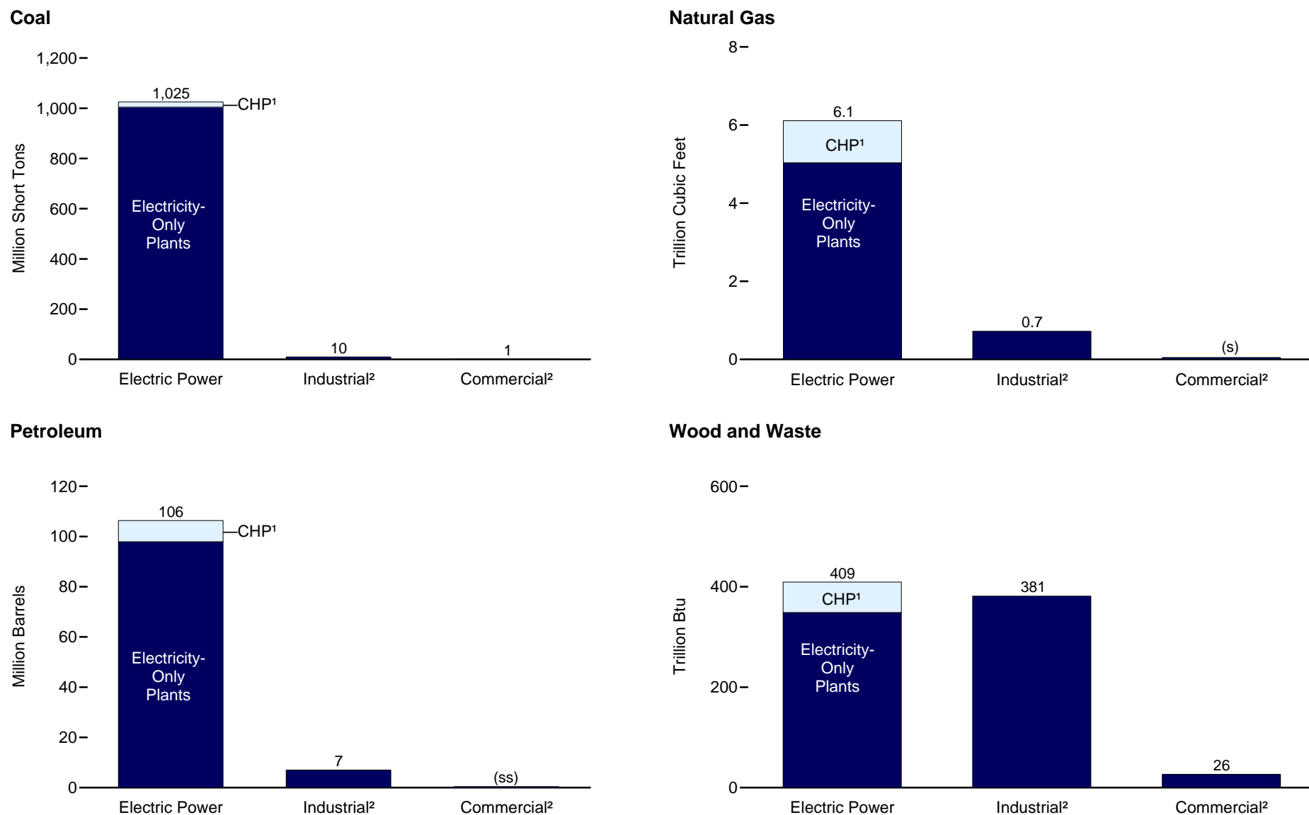
Figure 8.5b Consumption of Combustible Fuels for Electricity Generation by Sector, 2006
