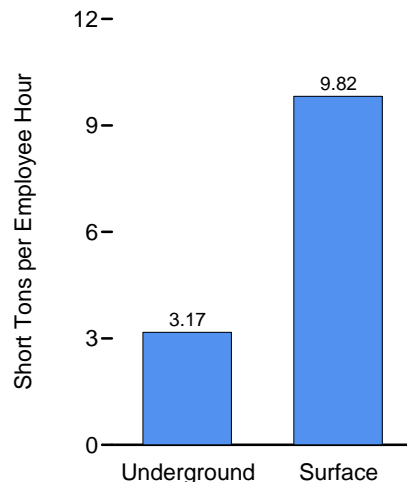
Mining Methods, 2008
