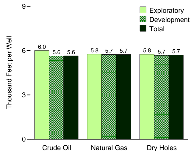
Average Depth, 2005
