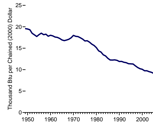
Energy Consumption per Real Dollar 2 of Gross Domestic Product, 1949-2006
