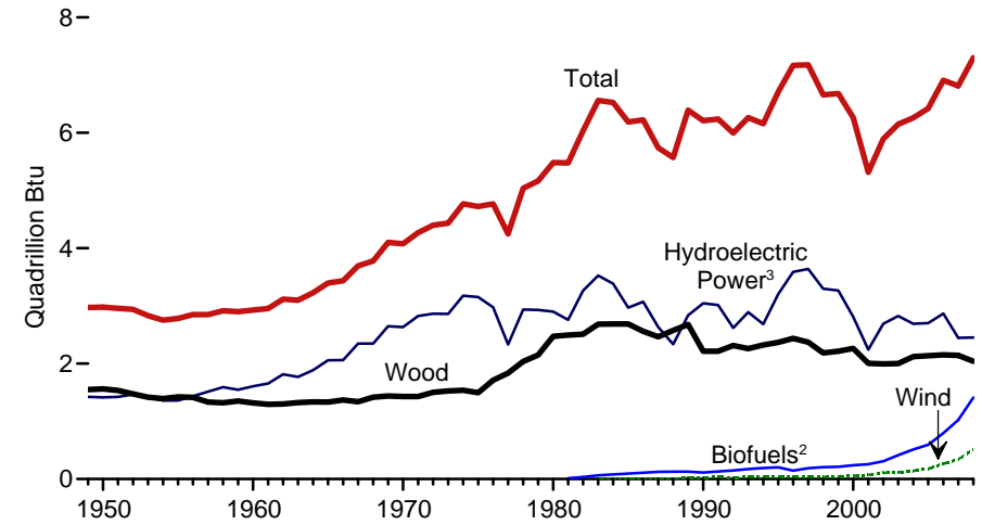
Renewable Energy Total Consumption and Major Sources, 1949-2008
