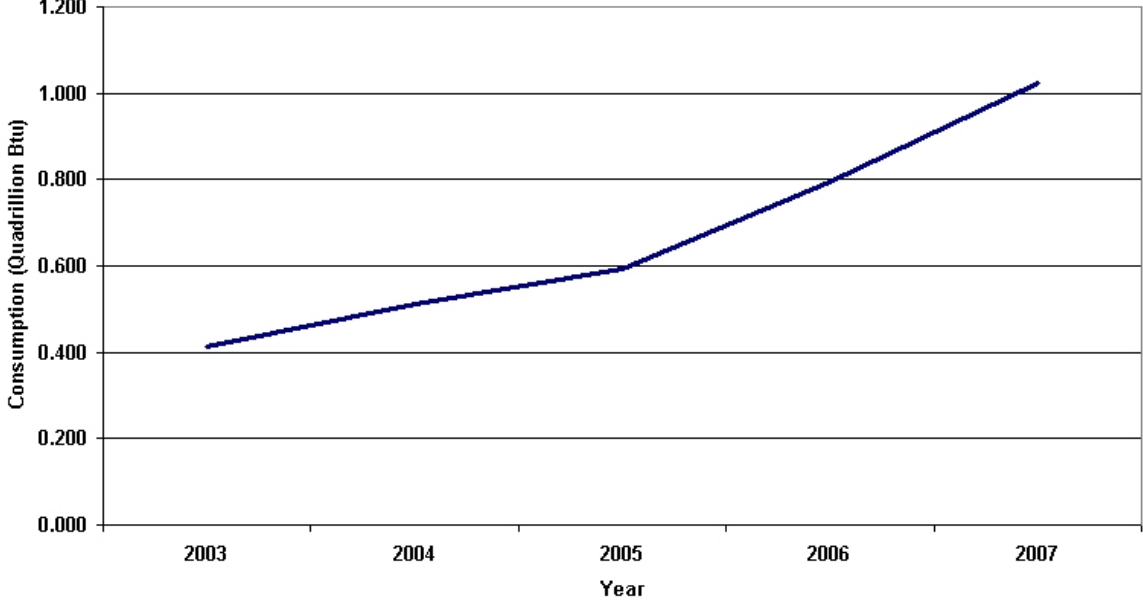
Figure 1.2 Biofuels Consumption, 2003-2007
