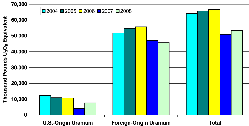
Figure 3. Uranium Purchased by Owners and Operators of U.S. Civilian Nuclear Power Reactors by Origin and Delivery Year, 2004-2008
