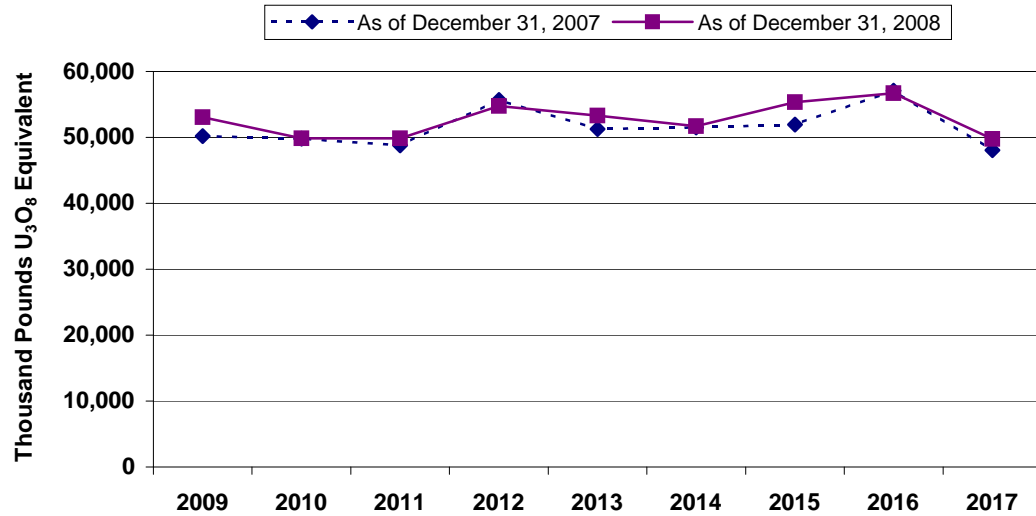
Figure 14. Shipments of Uranium Feed by Owners and Operators of U.S. Civilian Nuclear Power Reactors to Domestic and Foreign Enrichment Suppliers, 2009-2017
