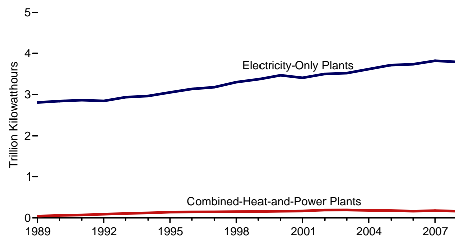
Electric Power Sector by Plant Type, 1989-2008
