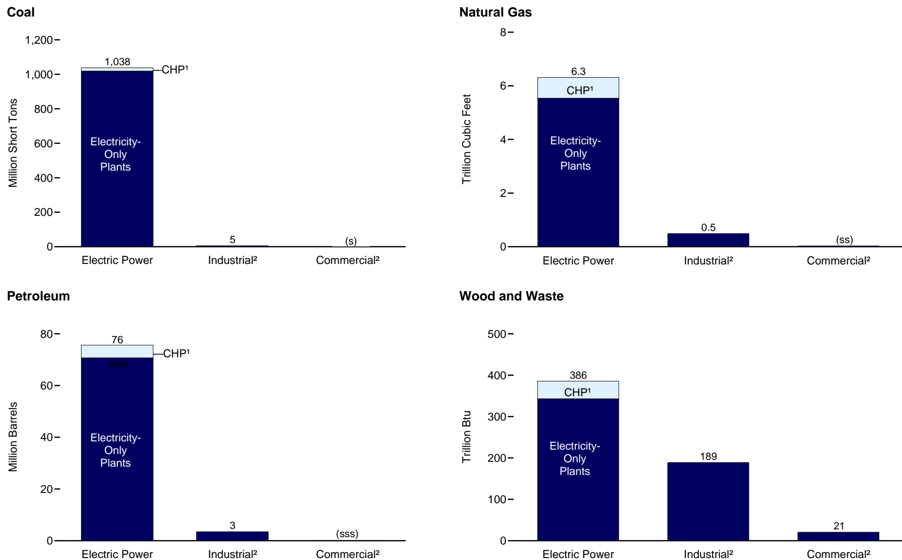
Figure 8.5b Consumption of Combustible Fuels for Electricity Generation by Sector, 2008
